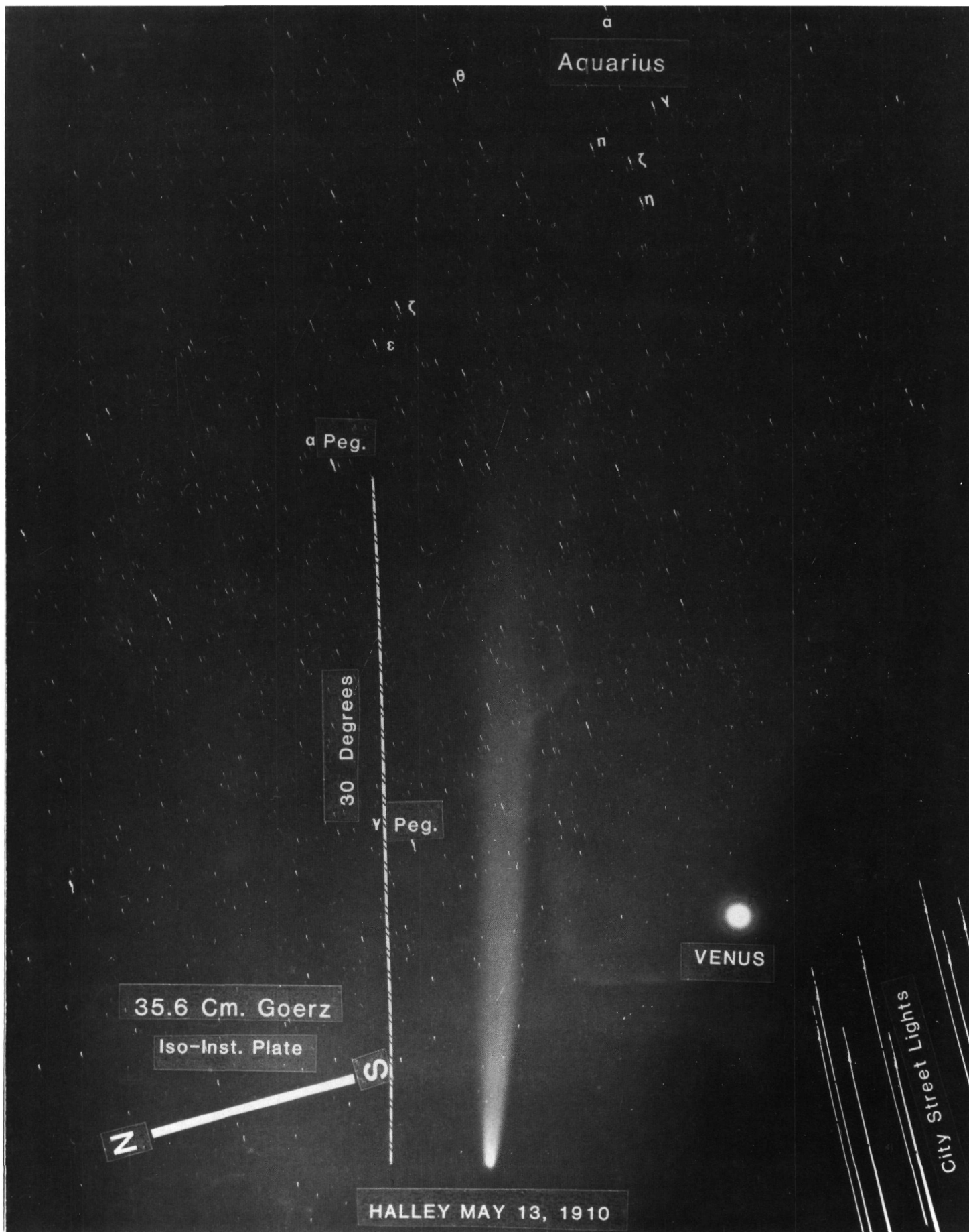
Figure 7. Photograph of Comet Halley obtained on May 13, 1910, with the 35.6-cm Goerz lens. Due to the longer f ratio, it does not show the comet's tail extending beyond Alpha Aquarius like the photographs obtained with the 17.8-cm Goerz and the 26.4-cm Cooke lenses.
